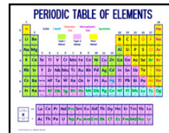
Periodic Table of Elements SCI057
