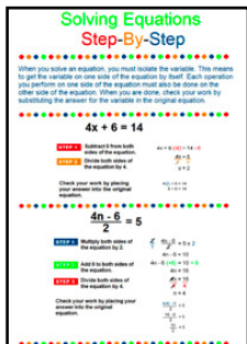
Solving Equations VIS385
