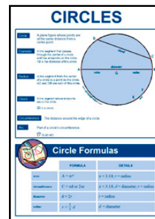
Parts of a Circle VIS360
