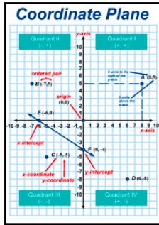
Coordinate Plane MTH018
