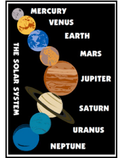
Solar System VIS501
