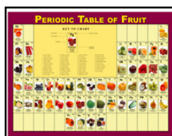
Periodic Table - Fruits SPE004
