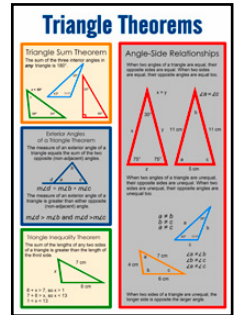
Triangle Theorems VIS486
