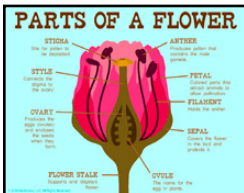
Parts of a Flower SCI023
