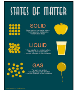
States of Matter SCI029
