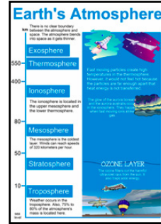
Earths Atmosphere VIS418
