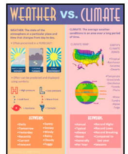
Weather Versus Climate SCI045
