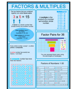
Factors and Multiples VIS461
