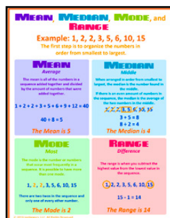
Mean Median Mode and Range MTH106
