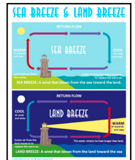
Sea Breeze and Land Breeze SCI051
