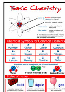
Basic Chemistry VIS492
