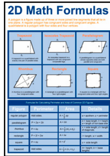
Area and Perimeter VIS357
