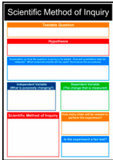
Scientific Method SCI004
