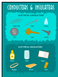
Conductors and Insulators SCI053
