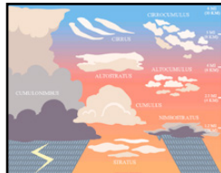
Cloud Types SCI021
