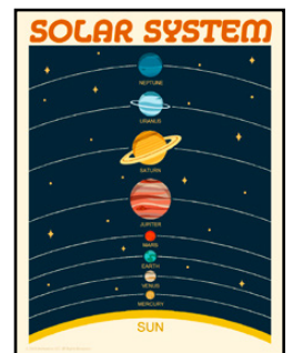
Solar System2 SCI025
