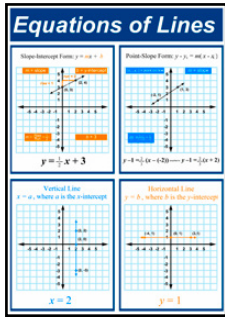
Equations of Lines MTH019
