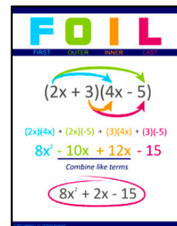
FOIL Method MTH080
