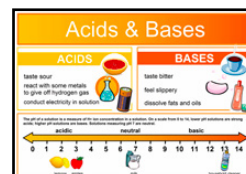
Acids and Bases SCI011
