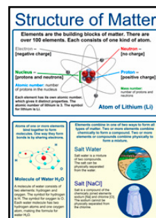
Structure of Matter VIS502
