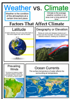
Weather vs Climate SCI009
