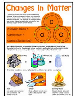
Changes in Matter SCI012
