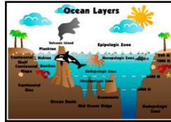
Ocean Layers VIS320
