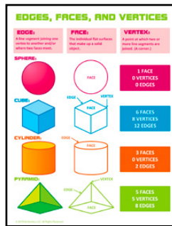
Edges, Faces, and Vertices MTH060
